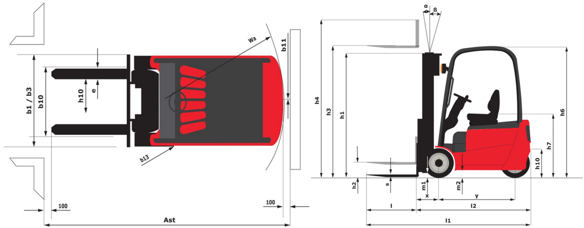
ME 318 - Dimensional drawing
