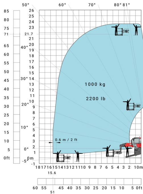
Machine on lowered stabilisers with 3D positive Metric
