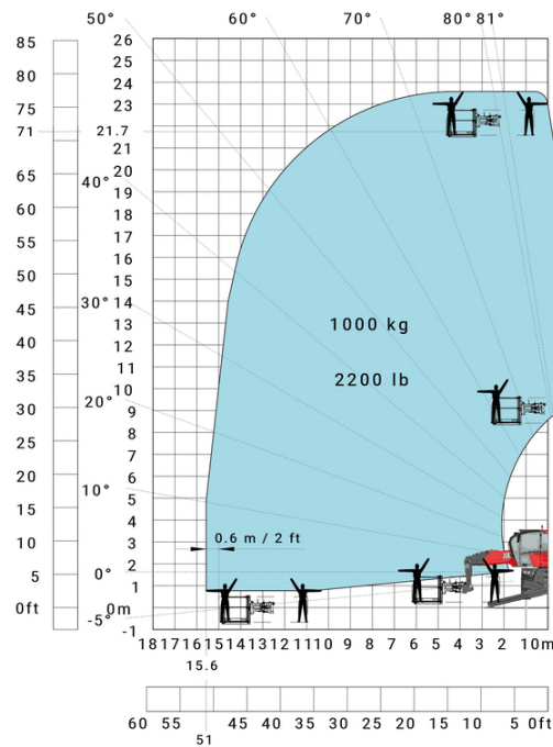
Machine on lowered stabilisers with 3D positive Imperial
